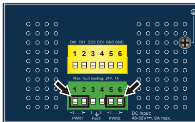
Figure 3-5: IGS-5225-4UP1T2S Upper Panel
