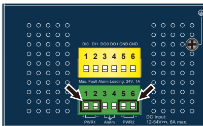
Figure 3-2: IGS-5225-8P4S-12V Upper Panel
