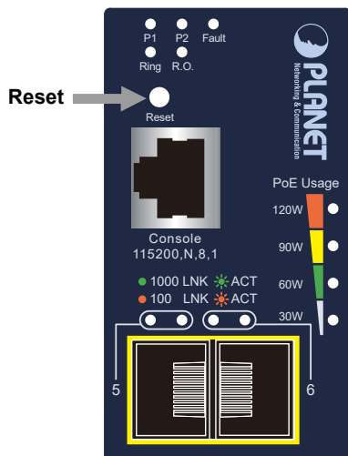
Figure 6-2: IGS-5225-4P2S Reset Button
